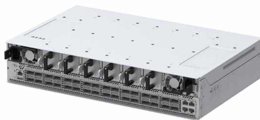
Figure 2: Celestica Edgestone™ Switch carrier-class top-of-rack switch includes NEBs compliance, is <300mm deep and offers all front-panel access to support constrained edge environments including central offices.
