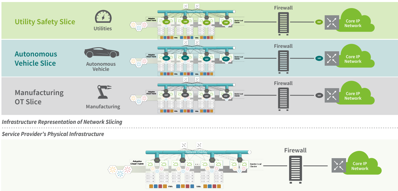
Figure 4: Network slicing has been designed into Netvisor ONE from the start, providing industry-leading slicing/segmentation across the data, control and management planes.
