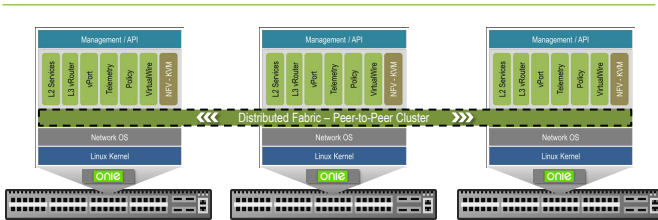
The Adaptive Cloud Fabric architecture clusters member switches into a symmetrical, unified operating domain
